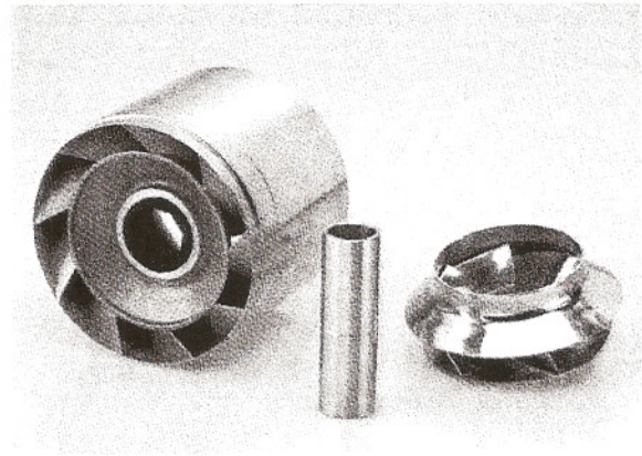
Mixed flow stage
