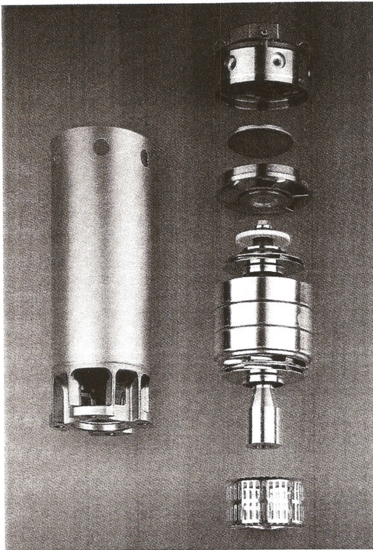
Radial flow stage
