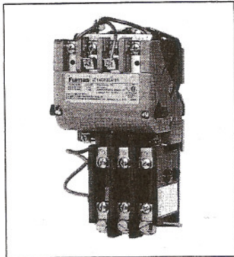
3 Phase, 3 Pole
